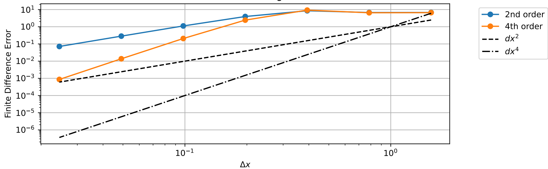
Demonstration of Convergence Order
