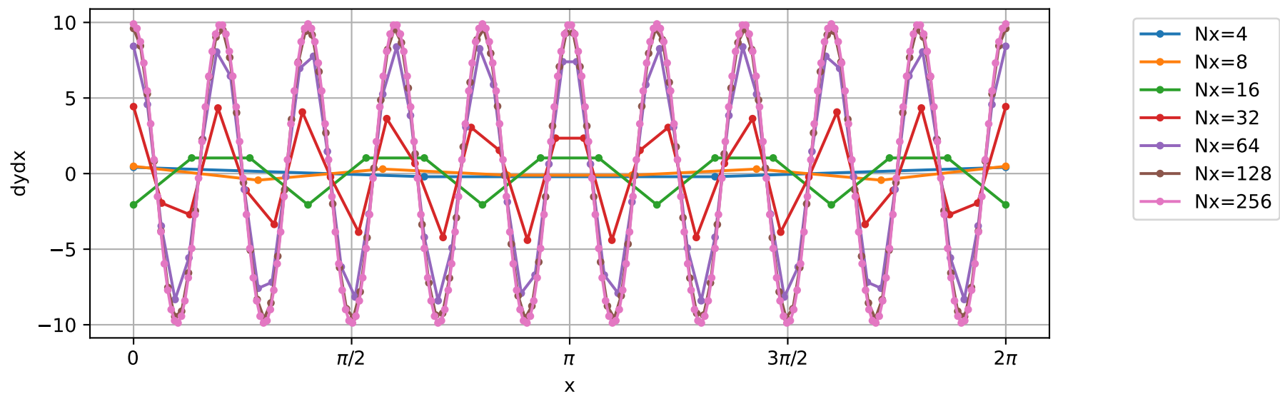
Order 2 Derivative
