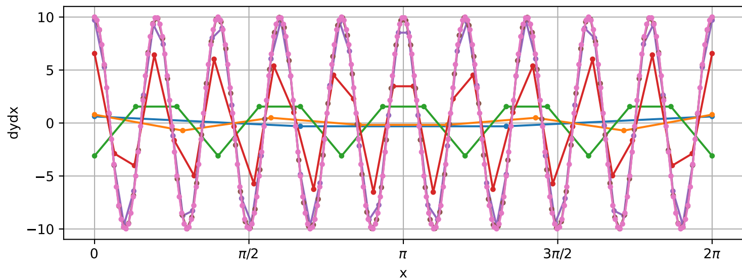
Order 4 Derivative
